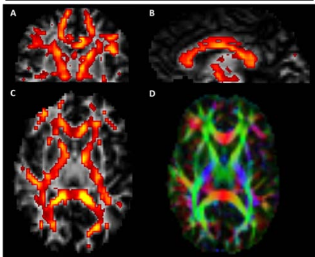
Figure 2: Tri-planar view (A-coronal, B-sagittal, C-axial) of the estimated average axon diameters d (overlay) and DTI-derived direction-encoded color (DEC) FA map (D).
