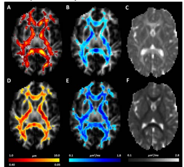
Figure 1: Microscopic anisotropy parameters estimated using qPFG diffusion MRI: average axon diameter d (A), intra-axonal water diffusivity D_{ax} (B), intra-axonal signal fraction f (D), and diffusivity of water in the unrestricted extra-axonal compartment D_{ex} (E) provide information complementary to DTI-derived metrics such as the axial (C) and radial diffusivity (F).
